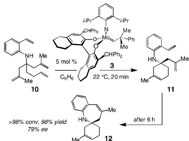
Scheme 2. Enantioselective Synthesis of Polycyclic Amines through Tandem Mo-Catalyzed ARCM/RCM
